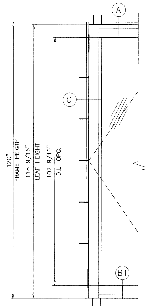
SINGLE OR DOUBLE DOORS WITH ADA SILL
